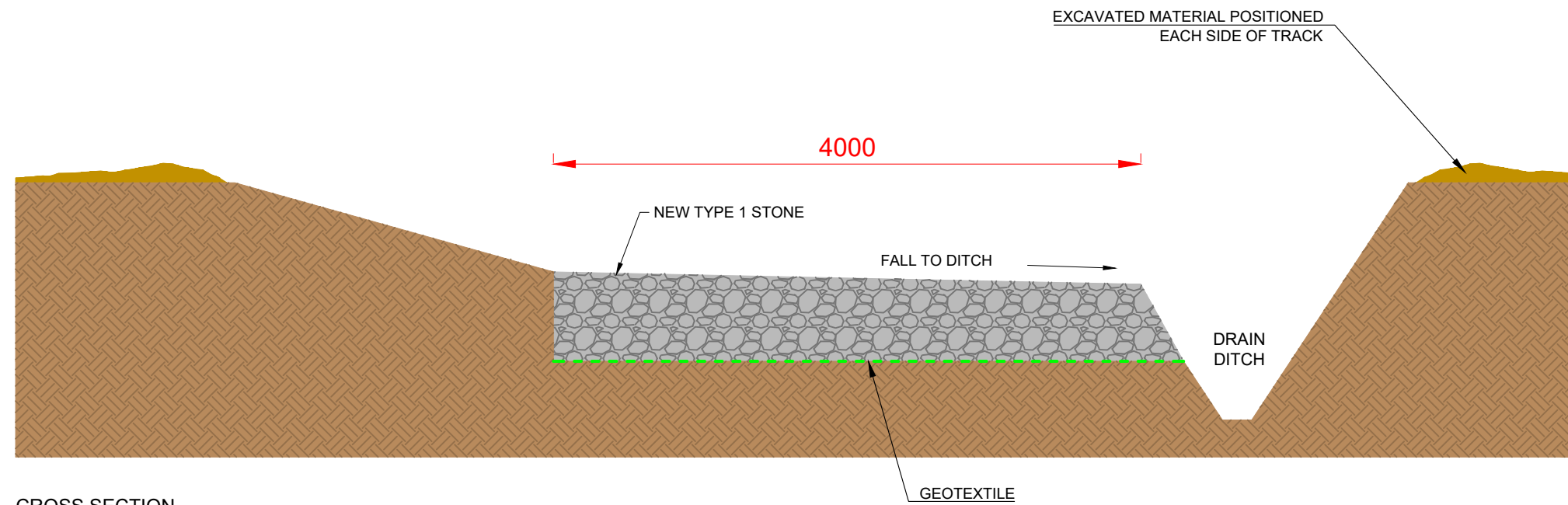
CROSS SECTION (Scale 1:40)
